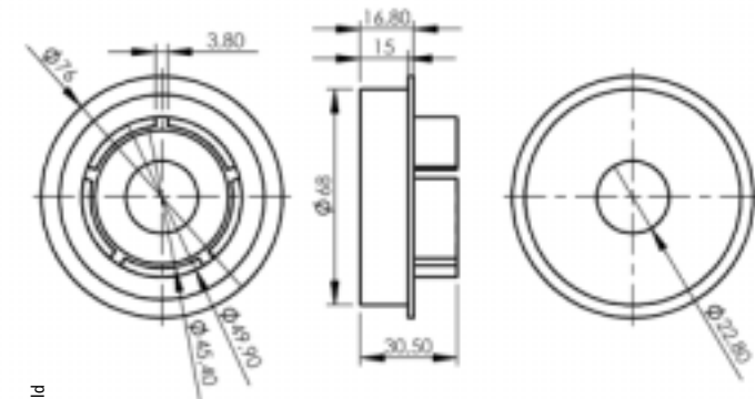
NA-BS68-8* Adapteri | Adapter NA-BS68-10* NA-BS68-12*
